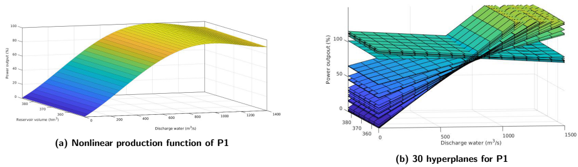
Figure 1: Comparison between the 2 production function models
