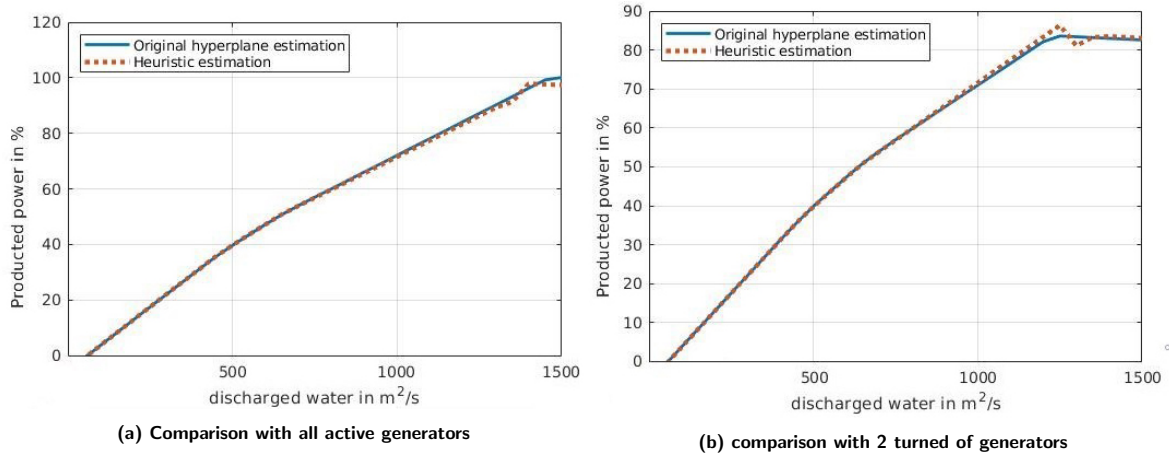
Figure 2: Comparison between the heuristic vs hyperplanes of the estimated production function
