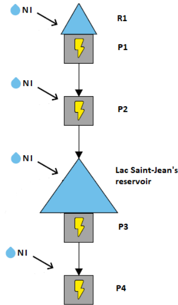
Figure 3: Saguenay lac Saint-Jean's hydropower system, where NI are Natural Inflows, P represent a power plant and R a reservoir
