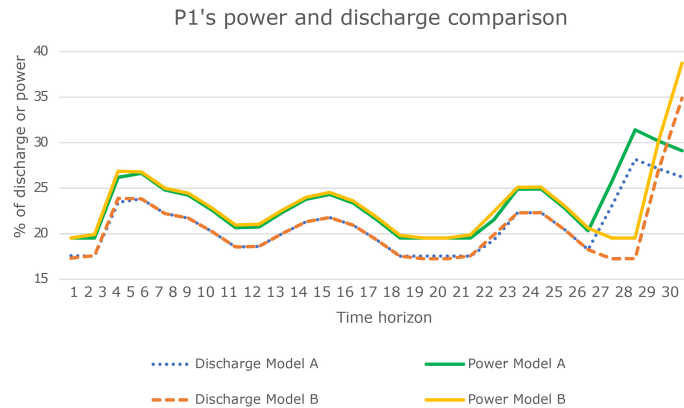
Figure 4: “P1” power and discharge comparison between both models for one instance
